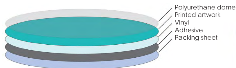
Components of a dome magnet
